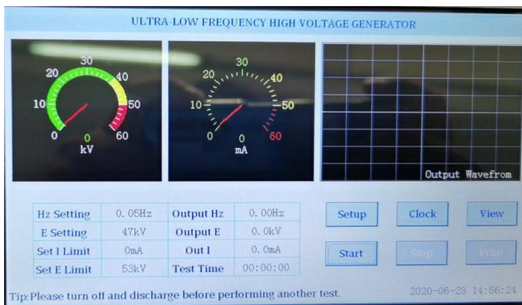
Figure 4 Schematic diagram of touch screen
