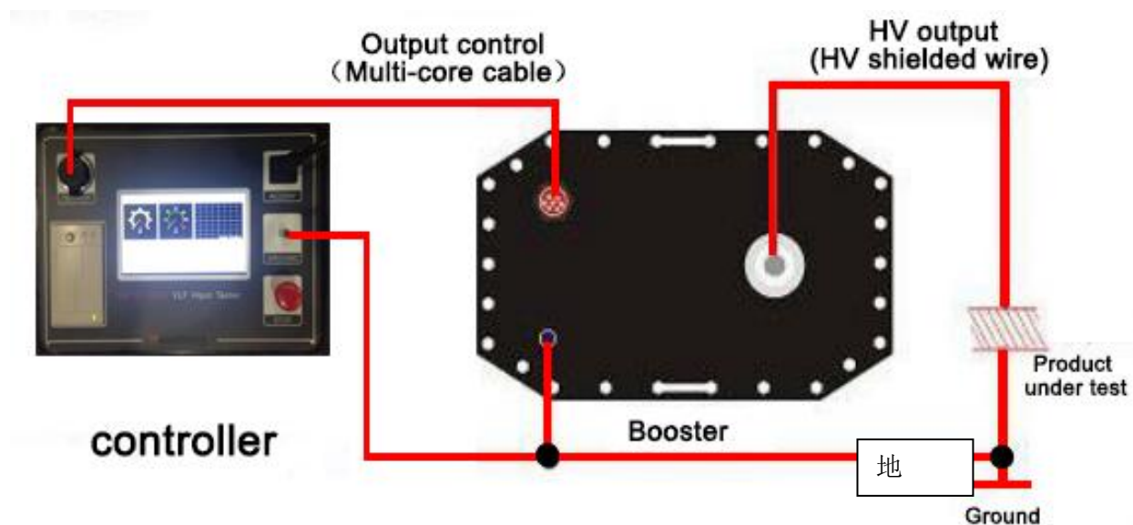
Figure 3 wiring diagram
