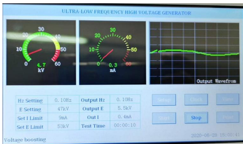
Figure 7 the controller indicates that the voltage is boosting
